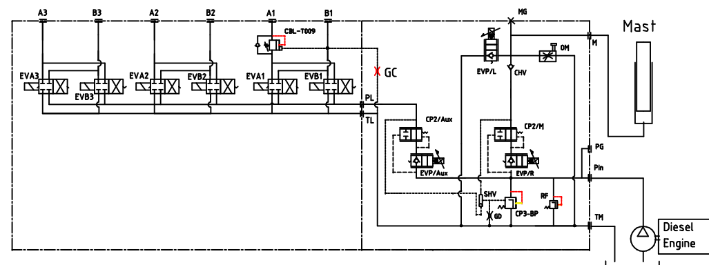
HYDRAULIC SCHEMATIC
