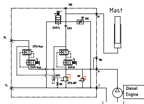
HYDRAULIC SCHEMATIC
